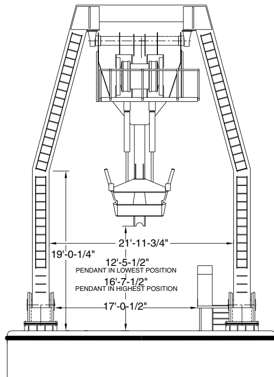
VIEW LOOKING FORWARD "A" FRAME IN VERTICAL POSITION
