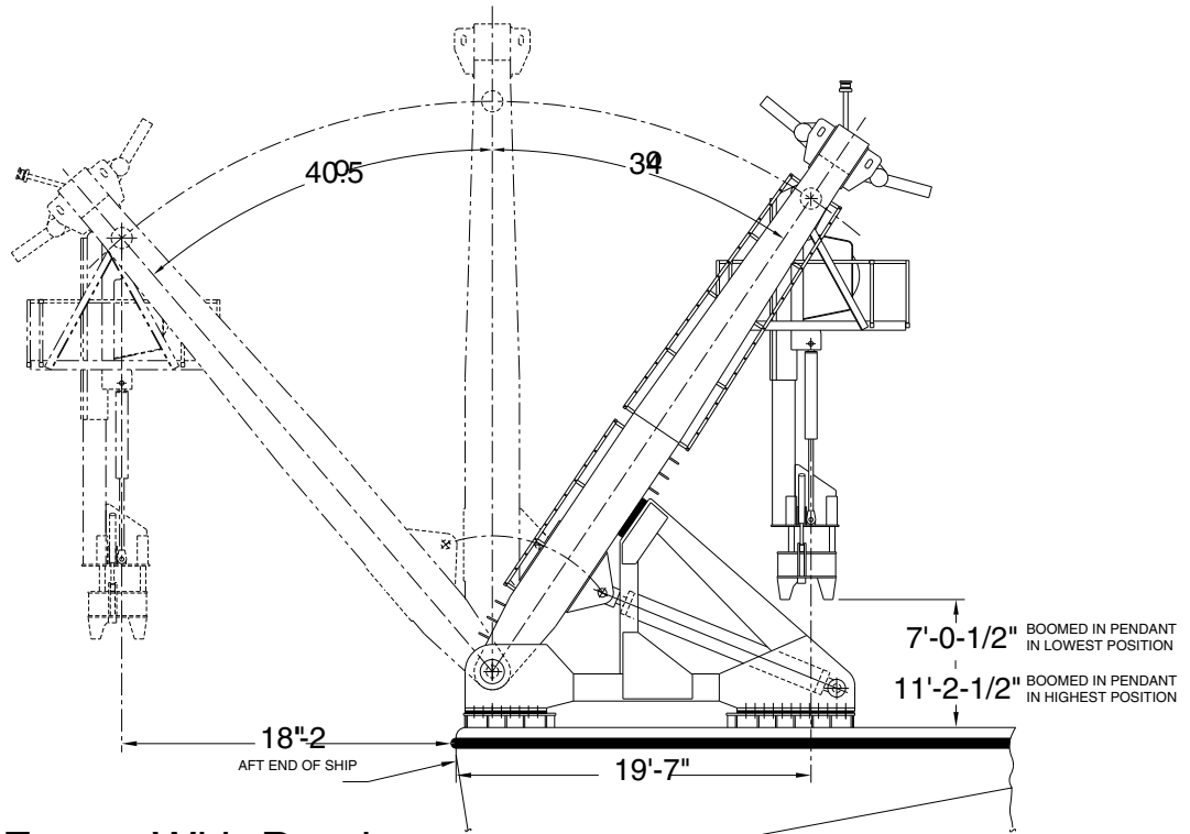
"A" Frame With Pendant
